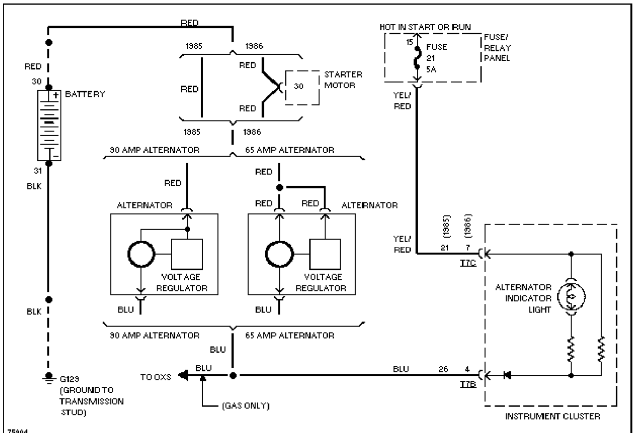
75904 Charging Circuit
