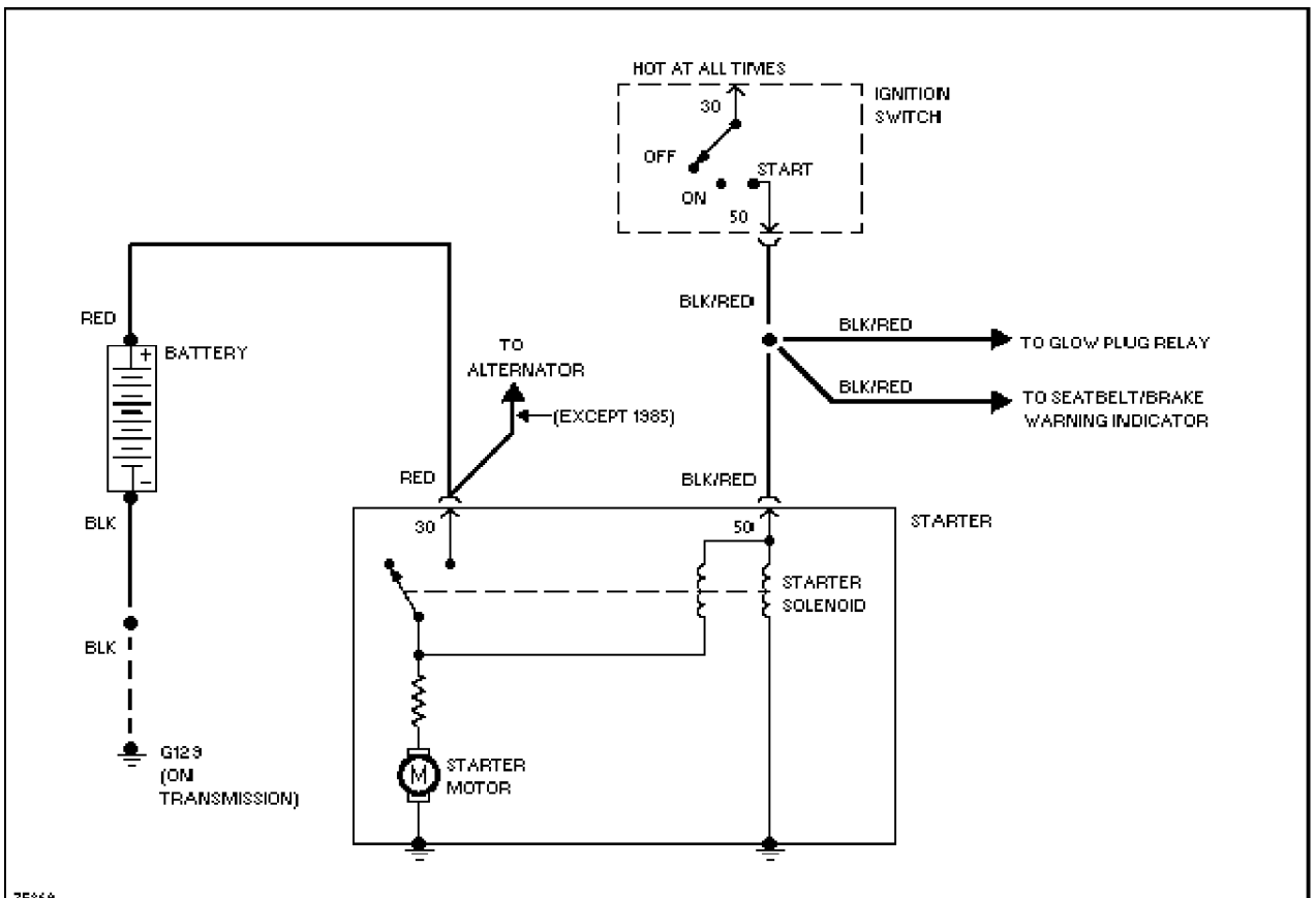
1.6L Diesel, Starting Circuit
