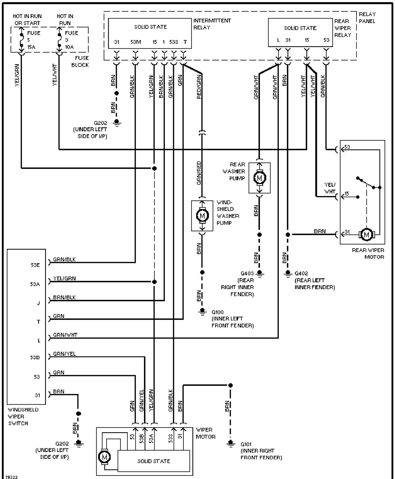
Wiper/Washer Circuit
