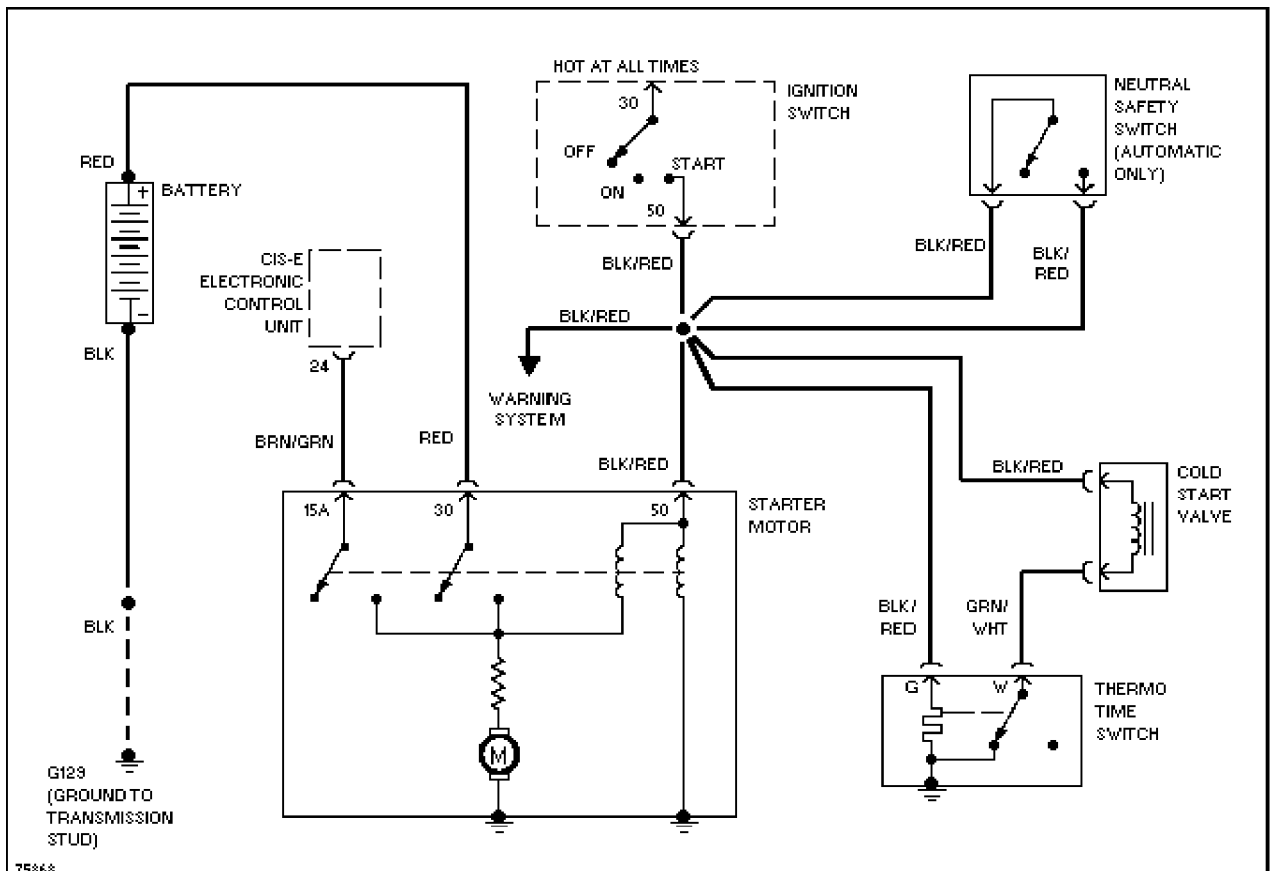
1.8L, Starting Circuit
