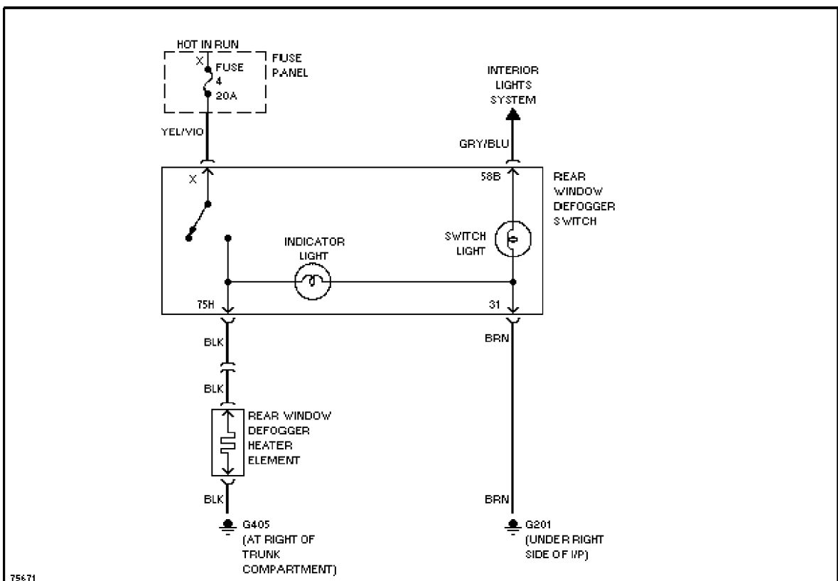
75671 Defogger Circuit
